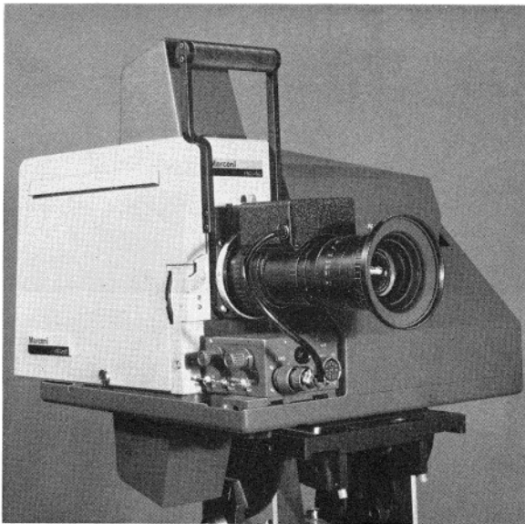
Camera and 7in viewfinder mounted on a standard head showing camera controls.
