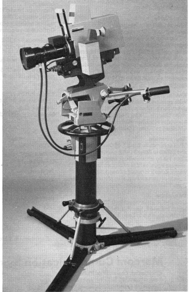
Camera mounted on Portaped with 10:1 manual zoom lens.
