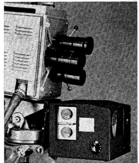
A Type BD 864 Broadcast Vidicon Camera with 'Minicue' attachment.
